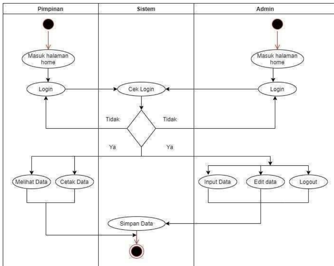
Gambar 2. Activity Diagram
