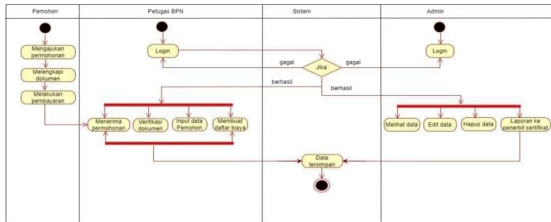
Gambar 3. Activity Diagram
