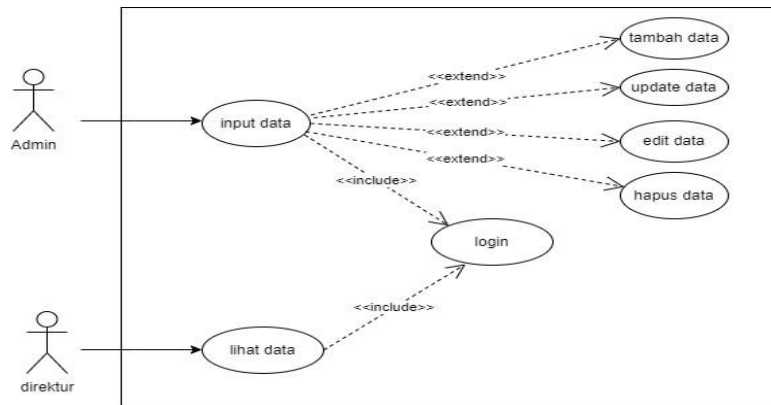
Gambar 2. Usecase diagram
