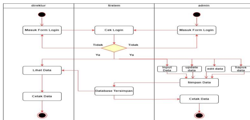
Gambar 3. Class Diagram
