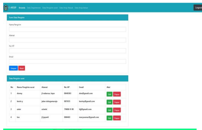
Gambar 9. Pengirim surat
