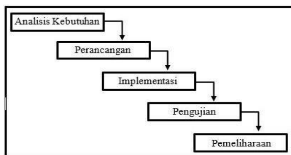
Gambar 1. Model waterfall
